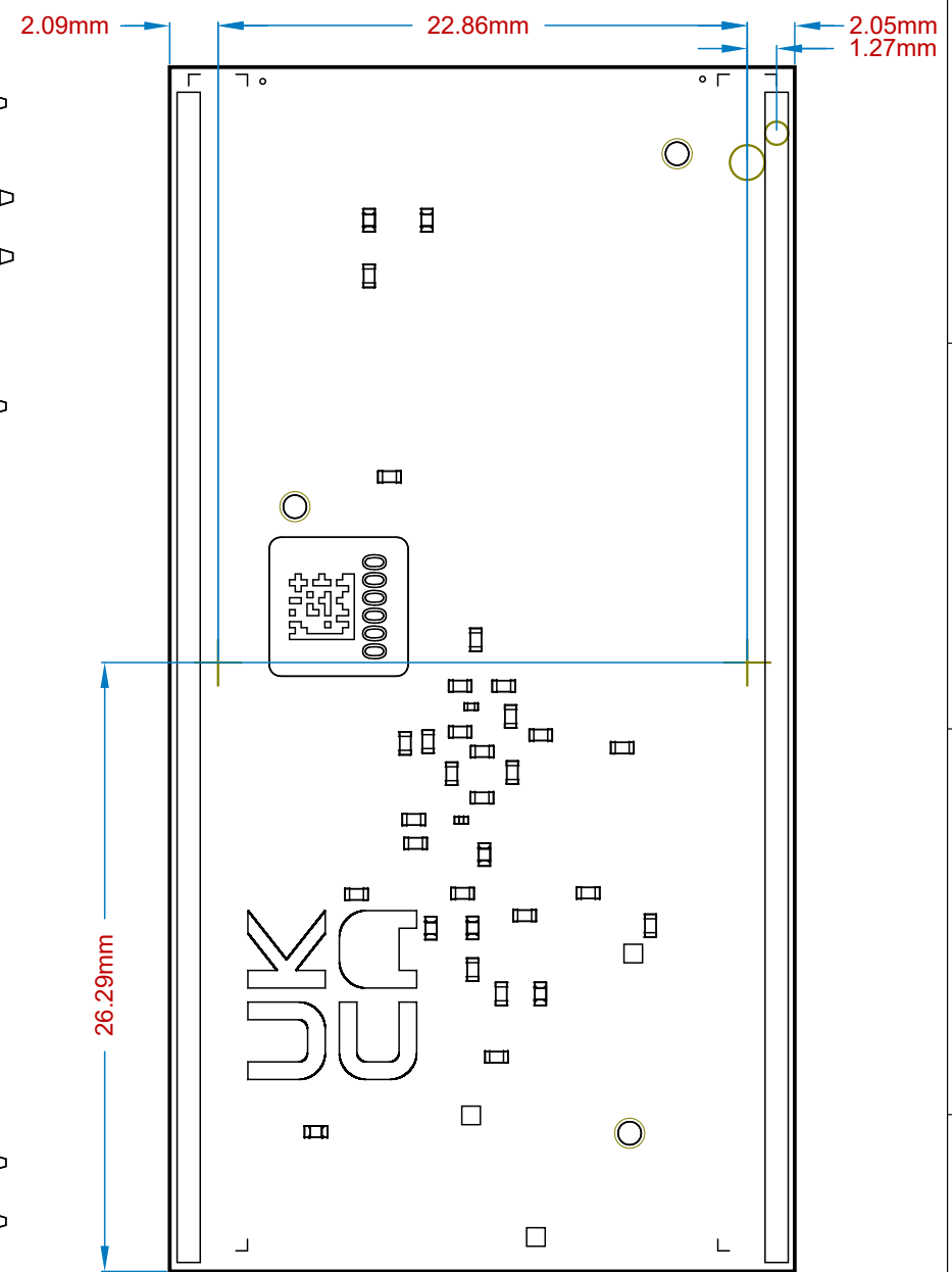
View from Bottom side (Scale 3:1)
