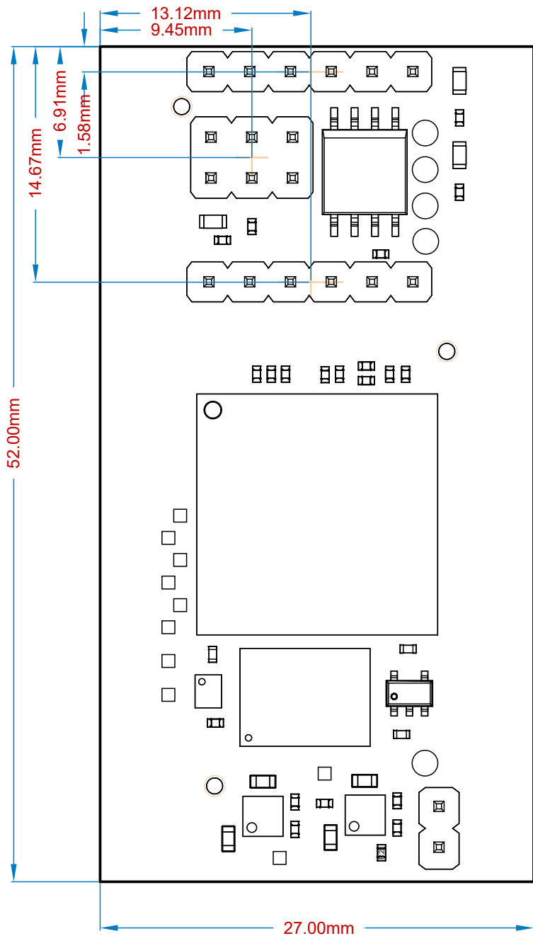
View from Top side (Scale 3:1)
