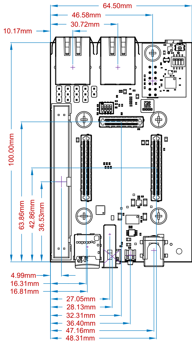
View from Top side (Scale 1:1)
