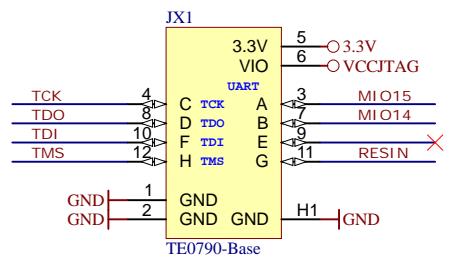
XMOD-FT2232H header: JTAG and UART
