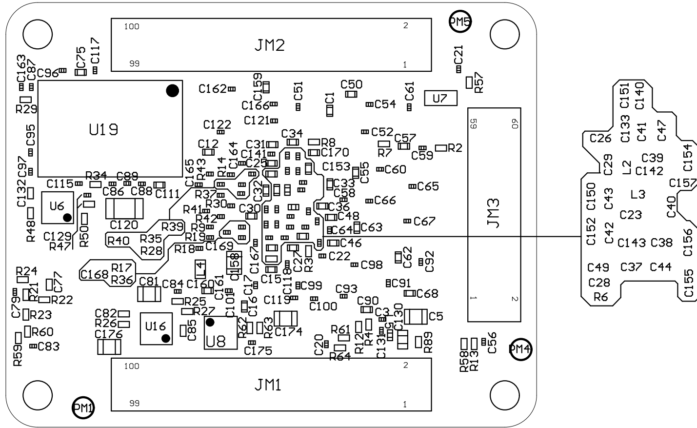
Bottom View
