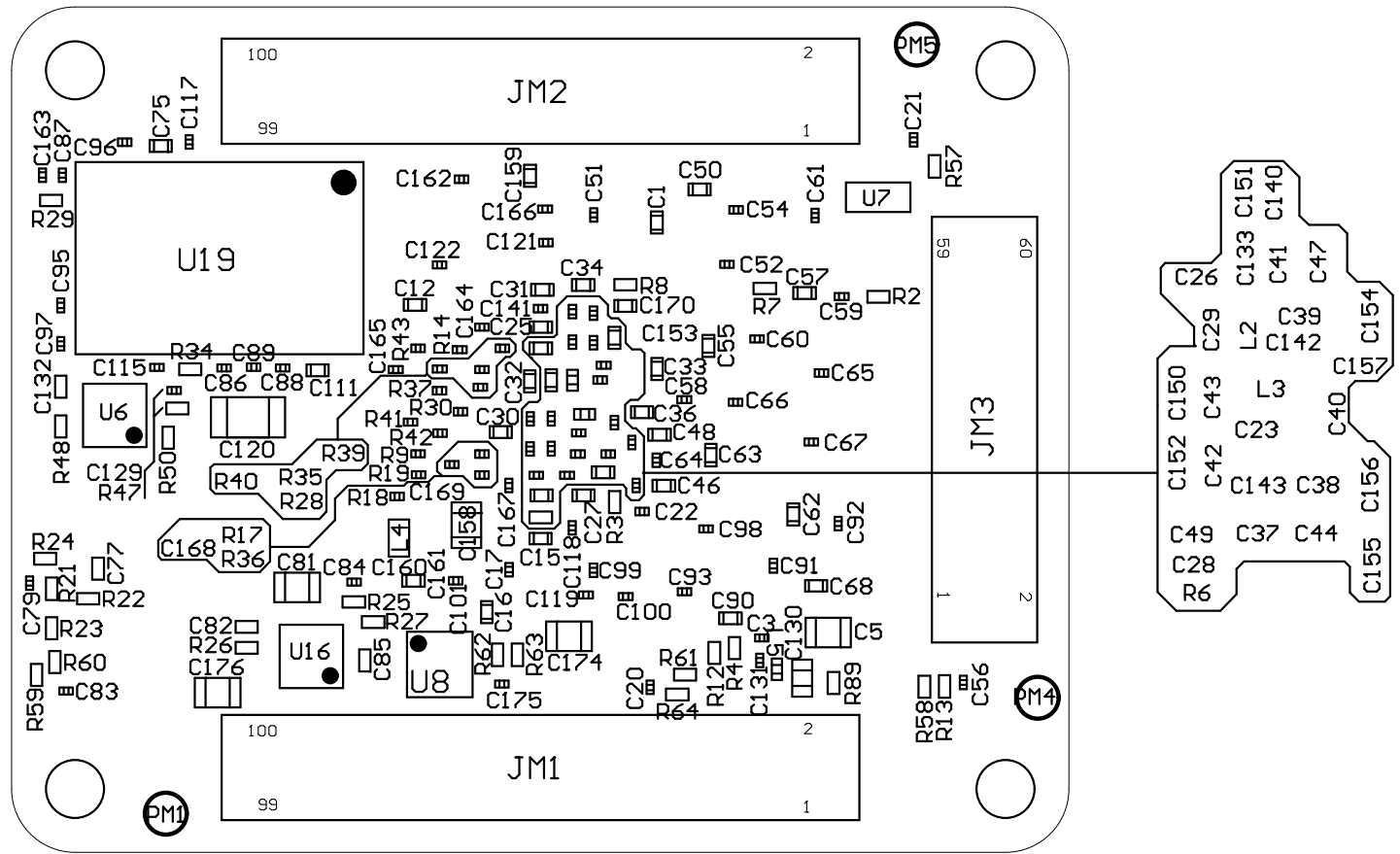
Bottom View
