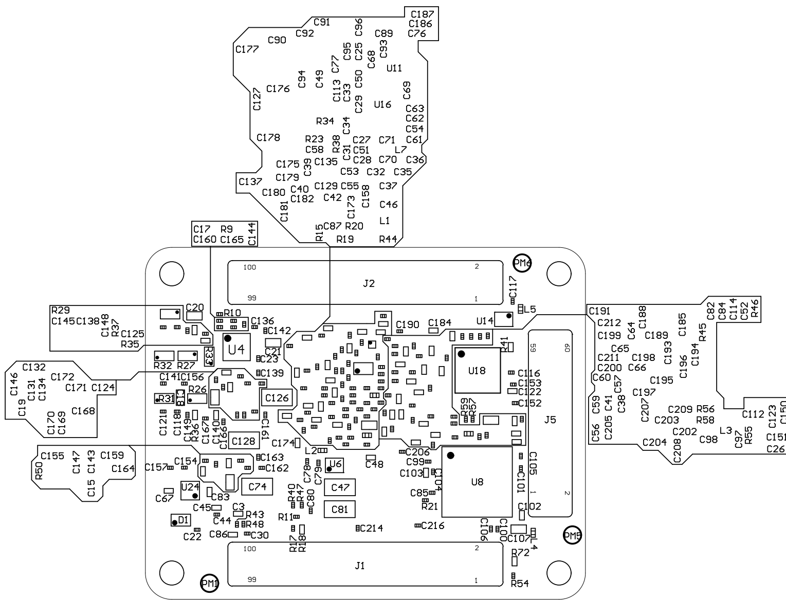
Bottom View
