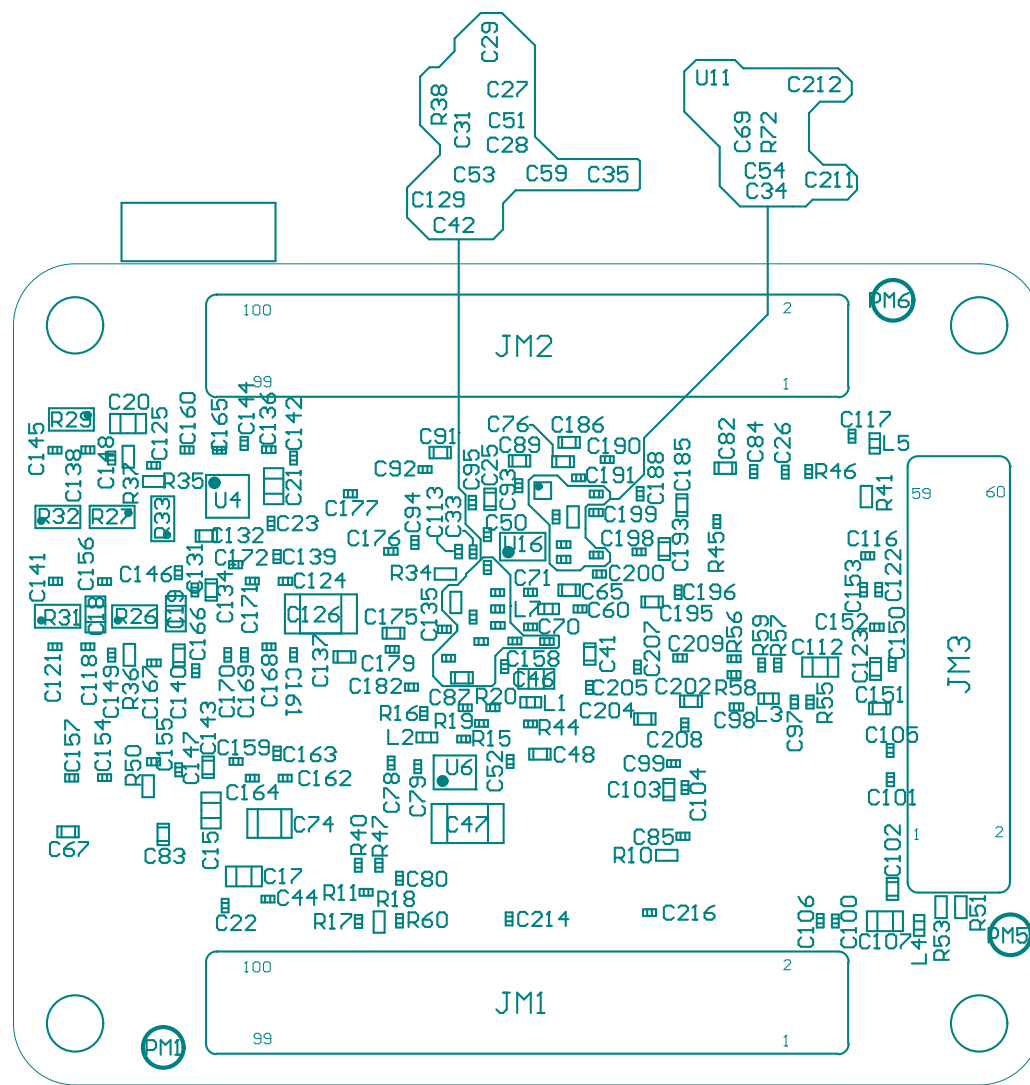
Bottom View
