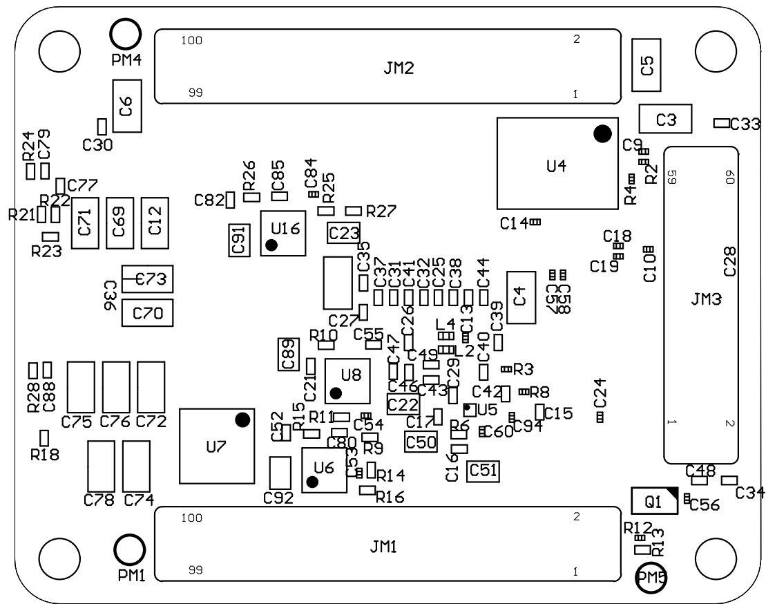
Bottom View
