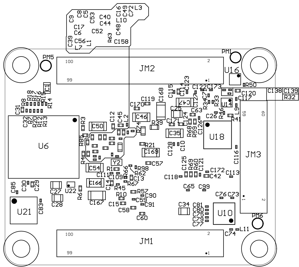
Bottom View
